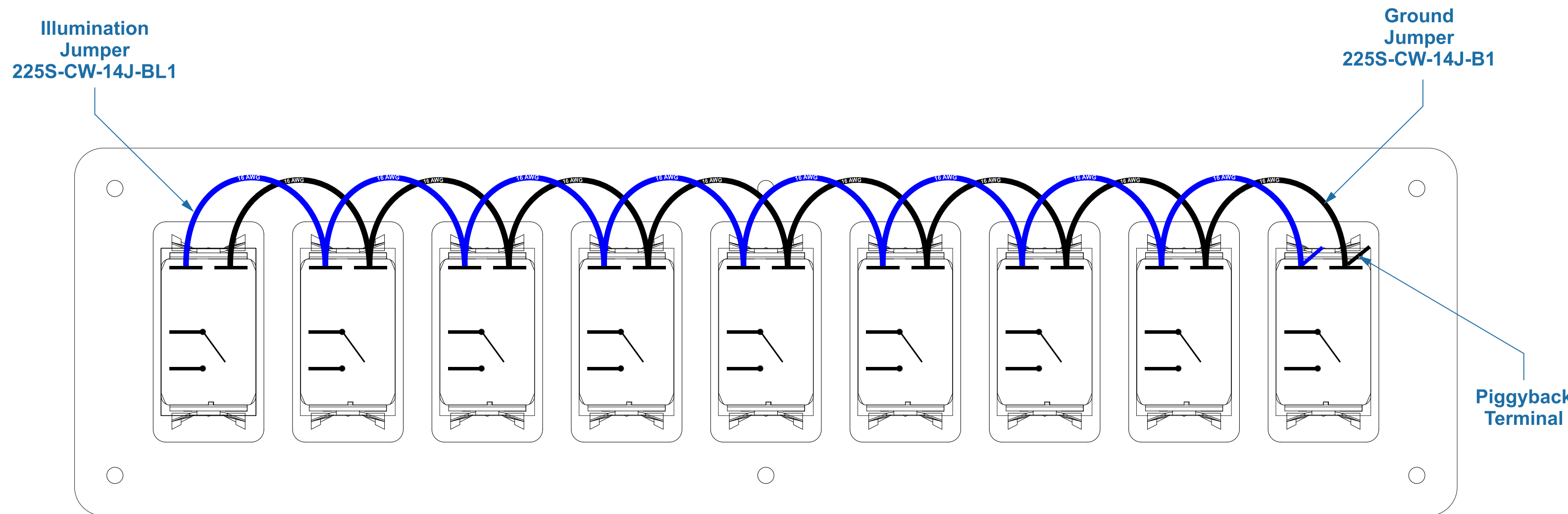
JUMPERS WIRING DIAGRAM
