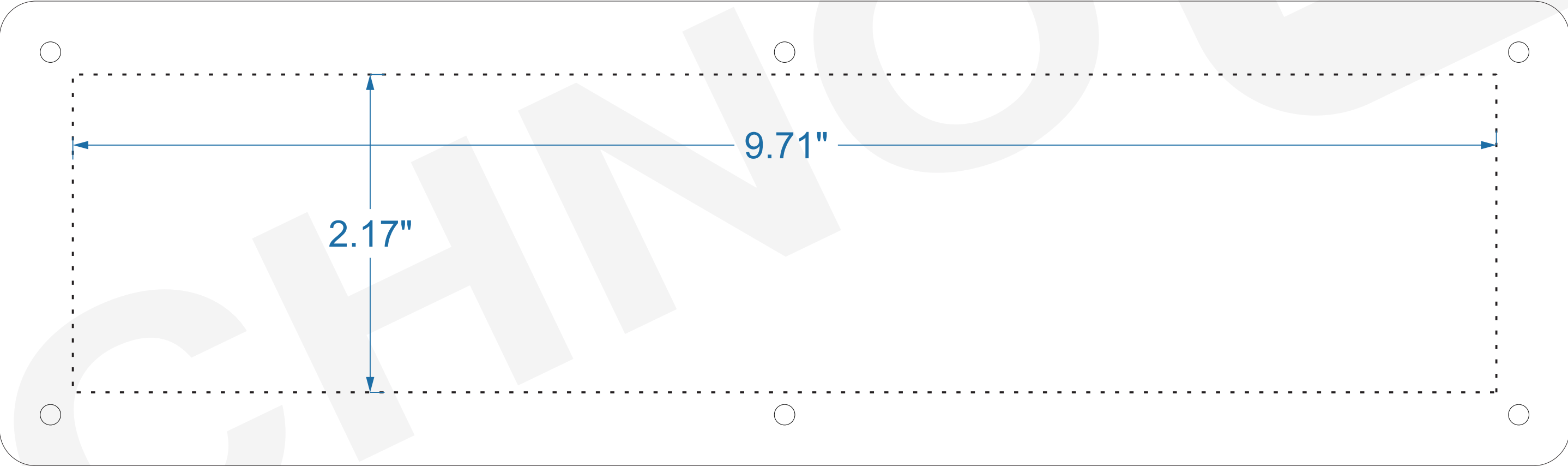
CUTOUT TEMPLATE (Not to scale)
