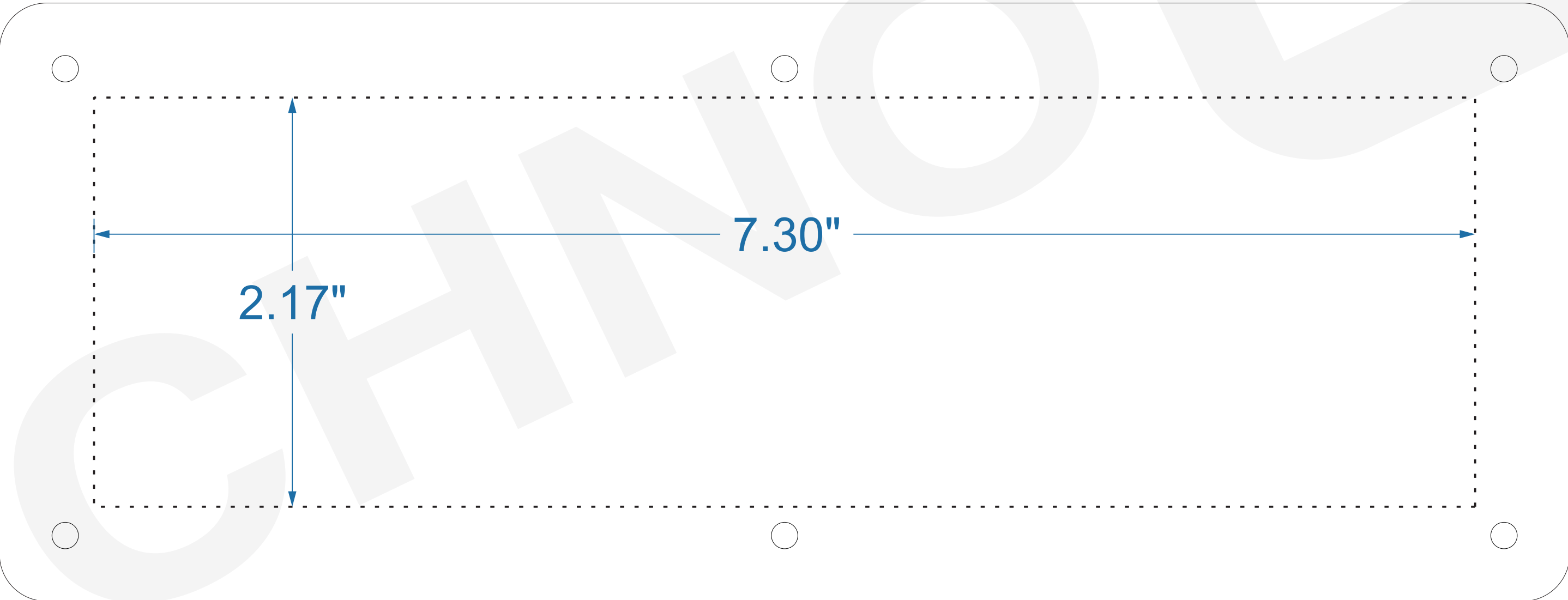
CUTOUT TEMPLATE (Not to scale)
