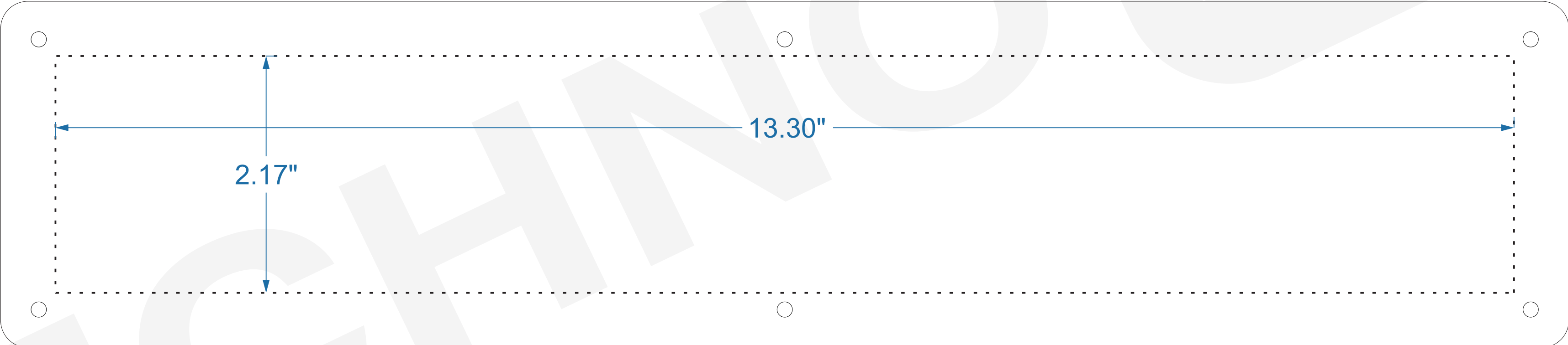
CUTOUT TEMPLATE (Not to scale)
