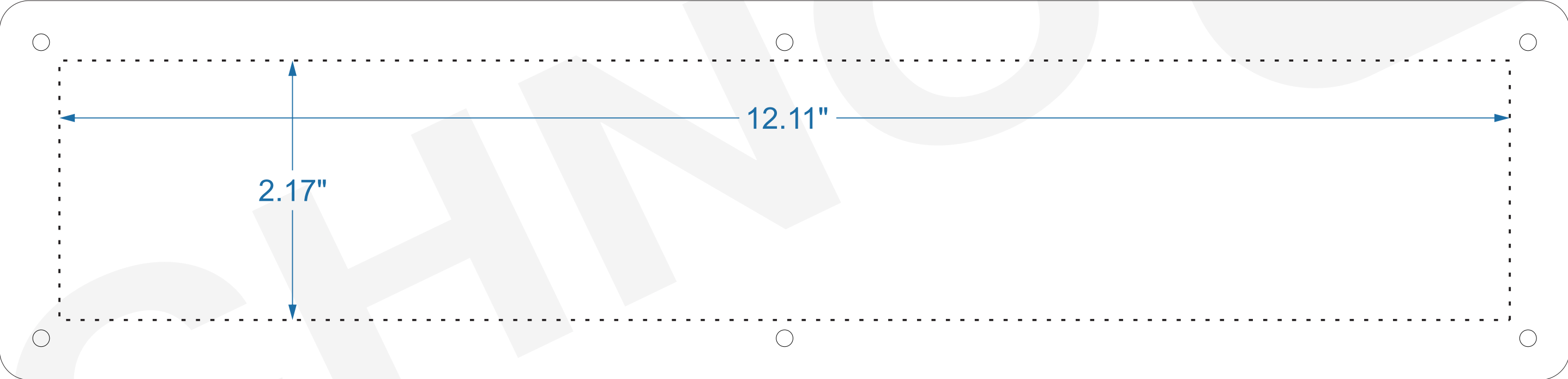
CUTOUT TEMPLATE (Not to scale)
